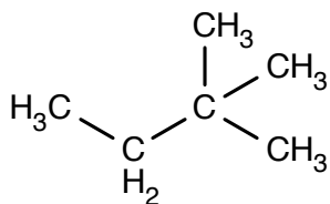
2,2-Dimethylbutaan
