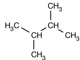
2,3-Dimethylbutaan
