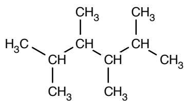
2,3,4,5-Tetramethylhexaan
