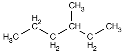
3-Methylhexaan
