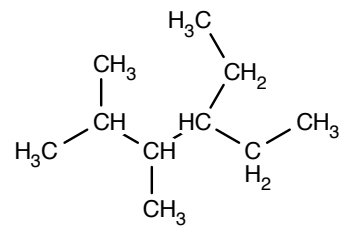
4-Ethyl-2,3-Dimethylhexaan
