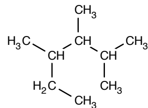
2,3,4-Trimethylhexaan
