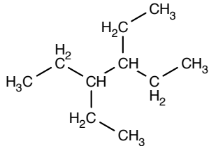
3,4-Diethylhexaan
