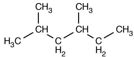
2,4-Dimethylhexaan
