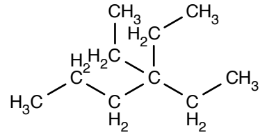
3,3-Diethylhexaan
