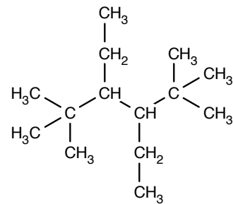
3,4-Diethyl-2,2,5,5-tetramethylhexaan
